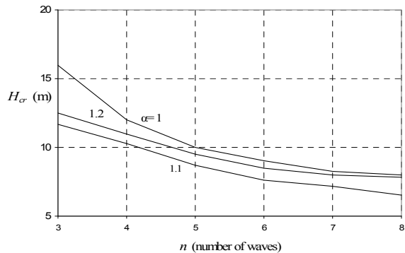
Fig. 16 : Required wave height for reaching the critical roll angle from an initial roll disturbance “around” 4.5°.
