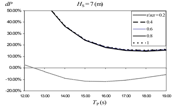
Fig. 24 : Difference in probabilities as the ratio r/z_{cr} is varied.
