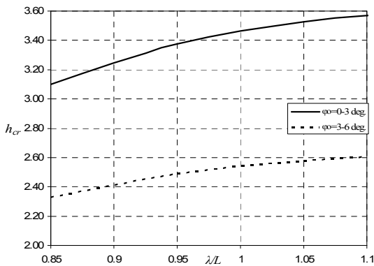
Fig. 17 : Critical values of h for pure-loss-of-stability.
